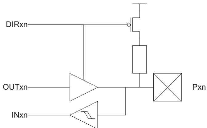
Figure 15-3. I/O Configuration - Totem-pole with Pull-up (on input)
