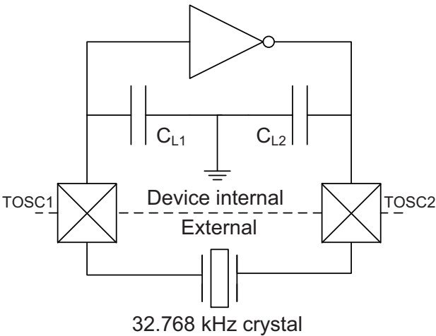
Figure 35-4. TOSC Input Capacitance
