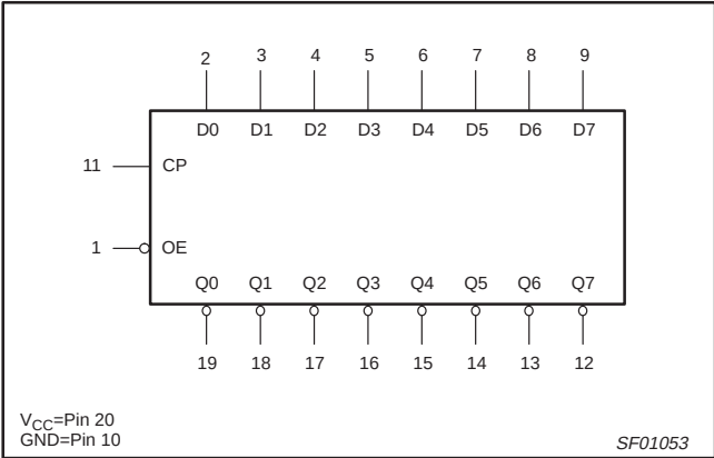
LOGIC SYMBOL – 74ALS564A
