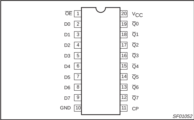
PIN CONFIGURATION – 74ALS564A
