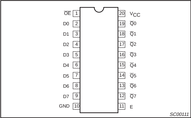
PIN CONFIGURATION – 74ALS563A
