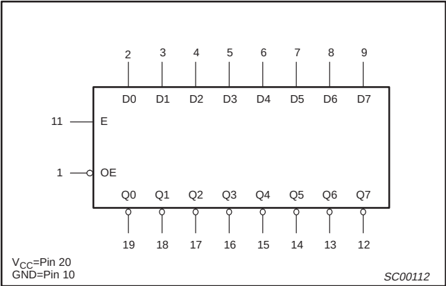
LOGIC SYMBOL – 74ALS563A
