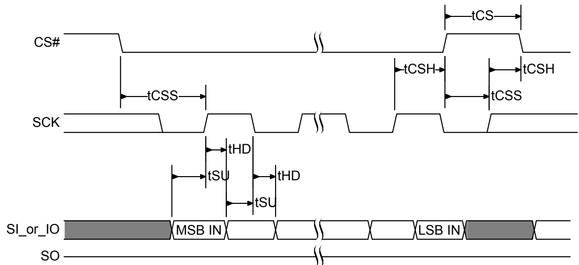
Figure 6.14 SPI DDR Input Timing
