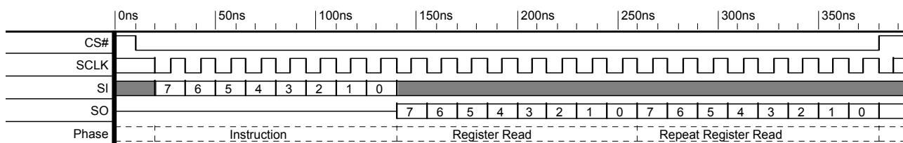
Figure 10.77 PPB Lock Register Read Command Sequence
