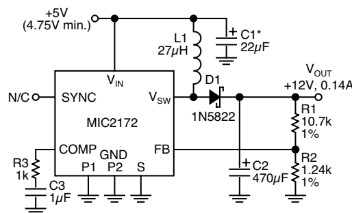
Figure 11. 5V to 12V Boost Converter
