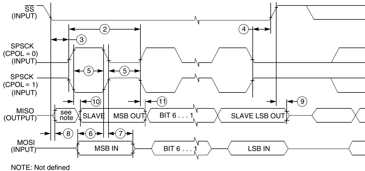
Figure 9. SPI slave mode timing (CPHA=1)
