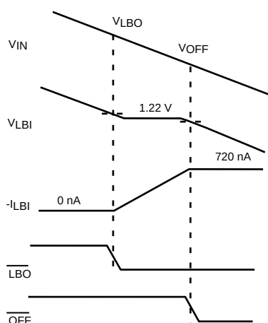
FIGURE 2: BATTERY MONITOR OPERATION GRAPHS
