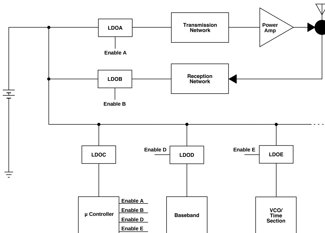
FIGURE 10: Linear regulators power up wireless application
