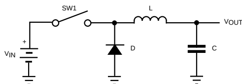
FIGURE 1: SIMPLE "BUCK" CONVERTER
