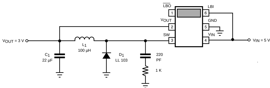
FIGURE 5: OPTIONAL SNUBBER
