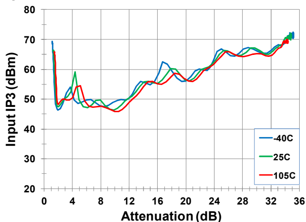
Input IP3 vs. Attenuation
