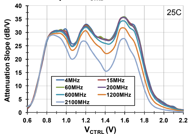
Attenuation Slope vs. V_{CTRL}
