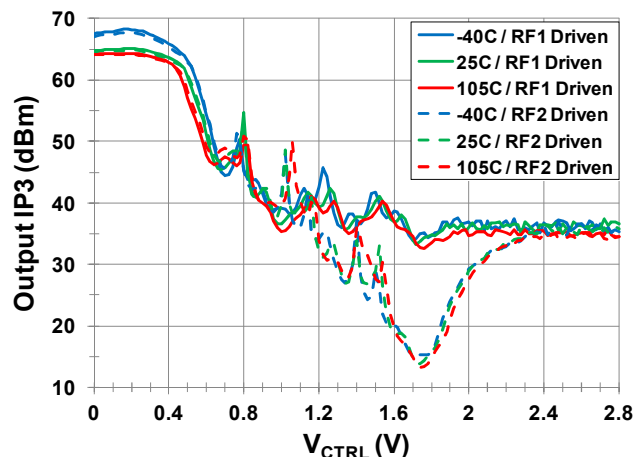
Output IP3 vs. V_{CTRL}
