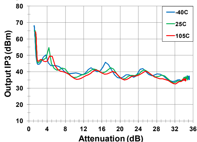
Output IP3 vs. Attenuation
