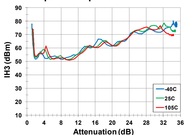
3 rd Harm Input Intercept Point vs. Attenuation
