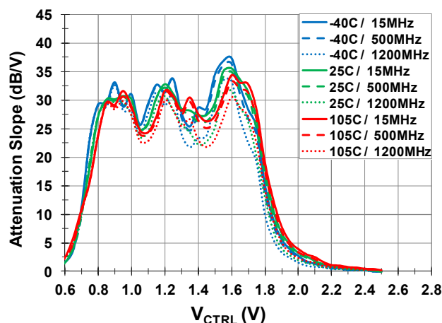
Attenuation Slope vs. V_{CTRL}
