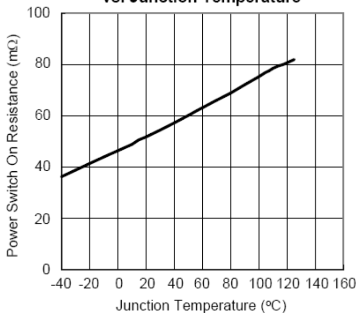
Power Switch On Resistance vs. Junction Temperature
