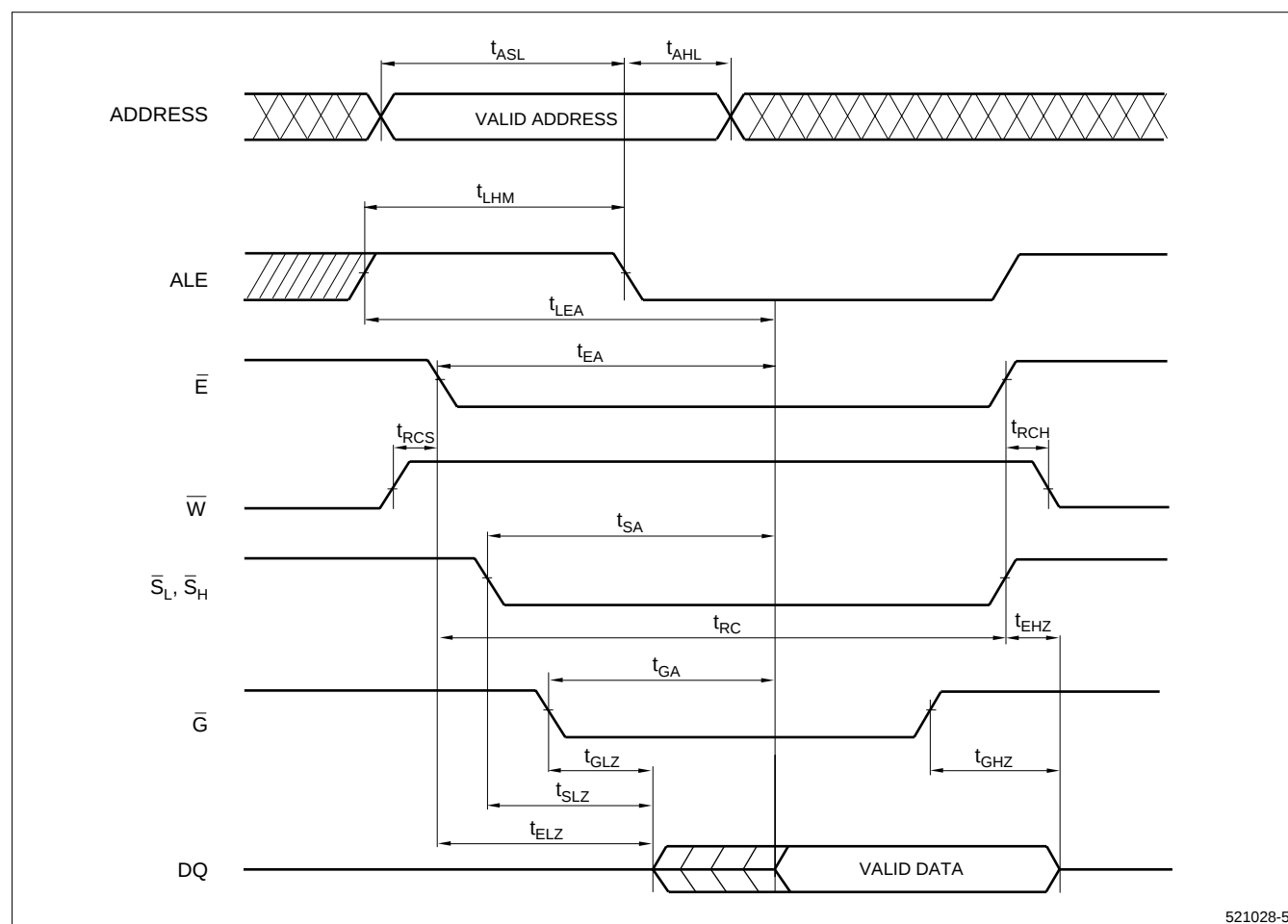
Figure 7. Read Cycle No. 4
