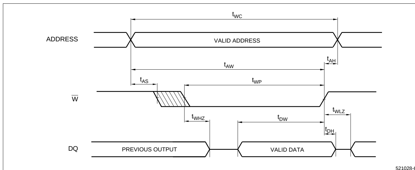
Figure 8. Write Cycle No. 1
