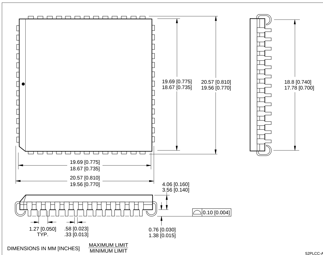
52-Pin PLCC
