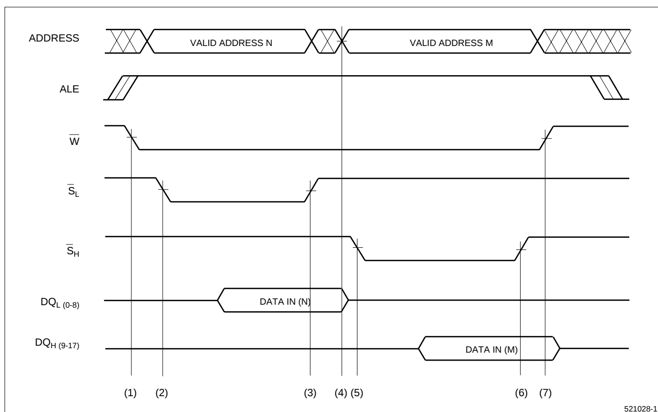
Figure 13. Byte Write ( \overline{E} is LOW)
