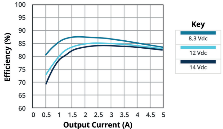
EFFICIENCY VS OUTPUT CURRENT VPOL5A-12-SMT (Vo = 1.5 Vdc)
