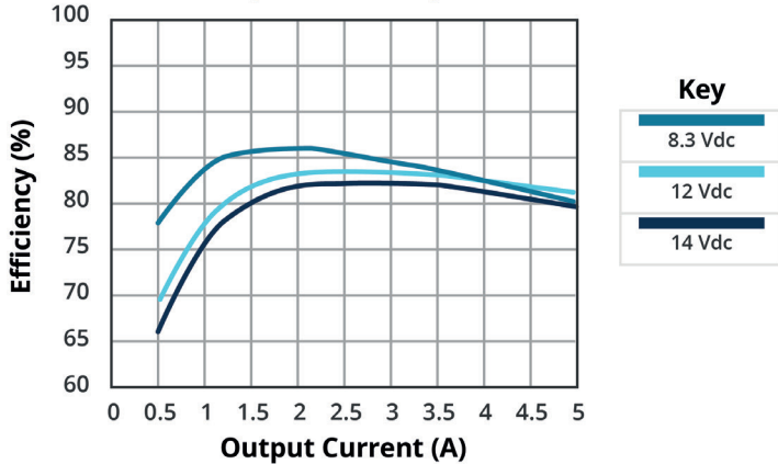
EFFICIENCY VS OUTPUT CURRENT VPOL5A-12-SMT (Vo = 1.2 Vdc)
