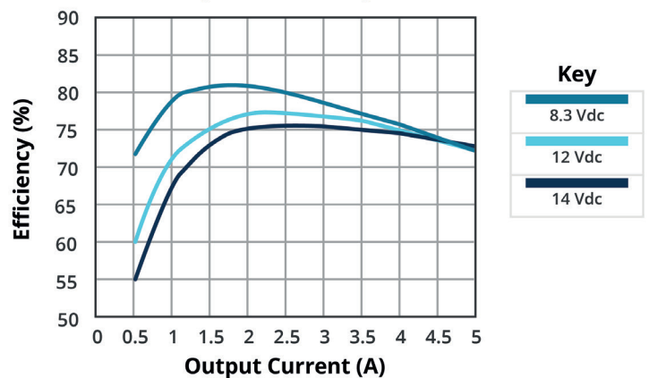
EFFICIENCY VS OUTPUT CURRENT VPOL5A-12-SMT (Vo = 0.75 Vdc)
