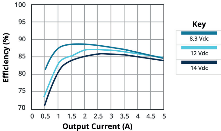
EFFICIENCY VS OUTPUT CURRENT VPOL5A-12-SMT (Vo = 1.8 Vdc)
