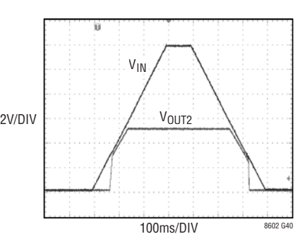
Channel 2 Start-Up and Dropout, R_L = 2\Omega
