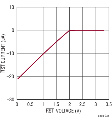
RST Pull-Up Current vs Voltage
