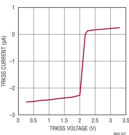
TRKSS Pull-Up Current vs Voltage
