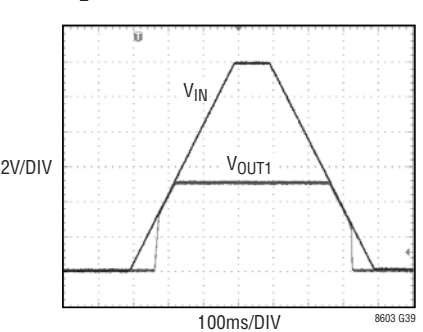
Channel 1 Start-Up and Dropout, R_L = 20\Omega
