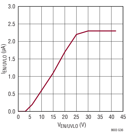
EN/UVLO Current vs Voltage
