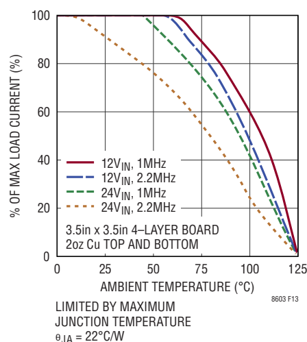
Figure 13. Thermal Derating, E- and I-Grade
