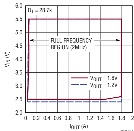
Channel 3 Full Frequency V_{IN} vs Load Current
