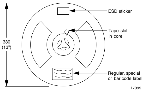
Fig. 12 - Tape and Reel Shipping Medium (EIA-481, revision A, and IEC 60286), 2000 units per reel
