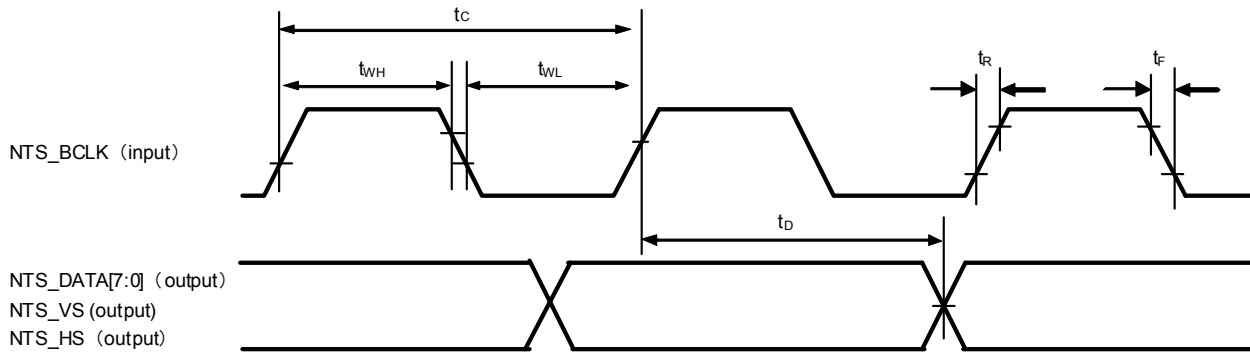
Figure 2-23. ITU-R BT.656 Interface Timing
