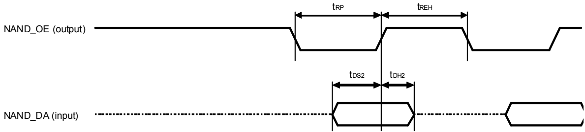
Figure 2-22. NAND Flash Interface Timing 2
