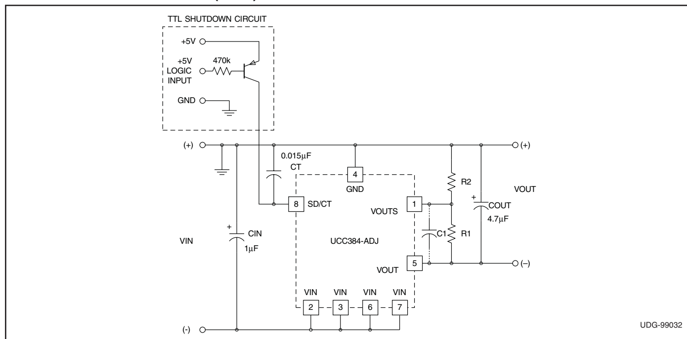
Figure 8. TTL controlled shutdown circuit for the UCC384.
