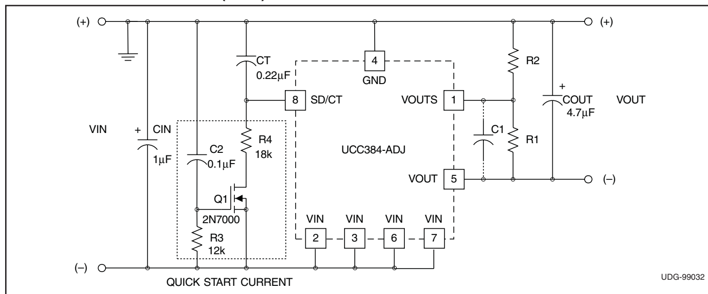
Figure 11. Quick start-up circuit for UCC384.
