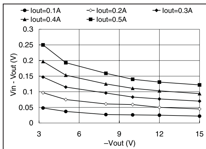
Figure 2. Dropout voltage vs. output voltage.
