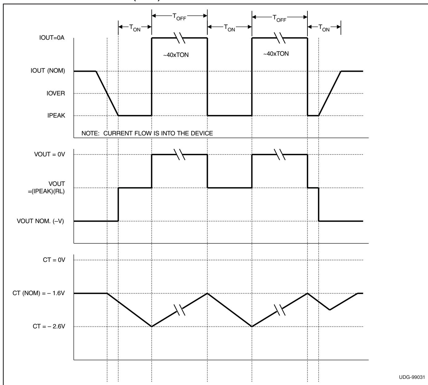
Figure 5. Short circuit timing.
