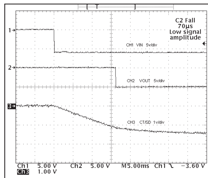
Figure 10. VIN to VOUT delay time during power-up with CT = 0.22μF.
