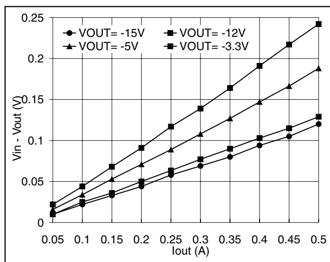
Figure 3. Dropout voltage vs. load current.
