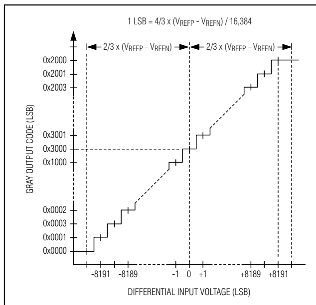
Figure 7. Gray-Code Transfer Function ( G/\overline{T} = 1 )
