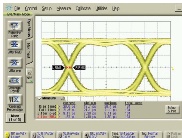
The N2101B eye output at 10.3125 Gb/s viewed on the DCA-J
