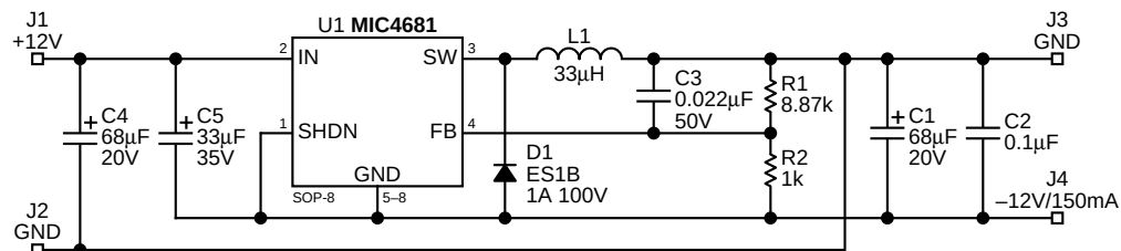
Figure 8. +12V to -12V/150mA Buck-Boost Converter
