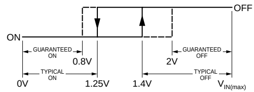
Shutdown Hysteresis
