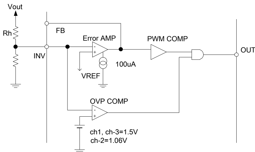
Figure 12. OVP Circuit
