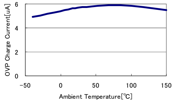
OVP Charge Current vs Ambient Temperature
