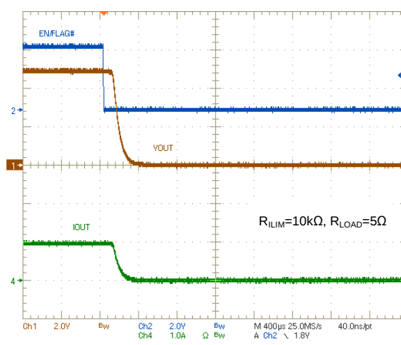
Disable with 5Ω Load
