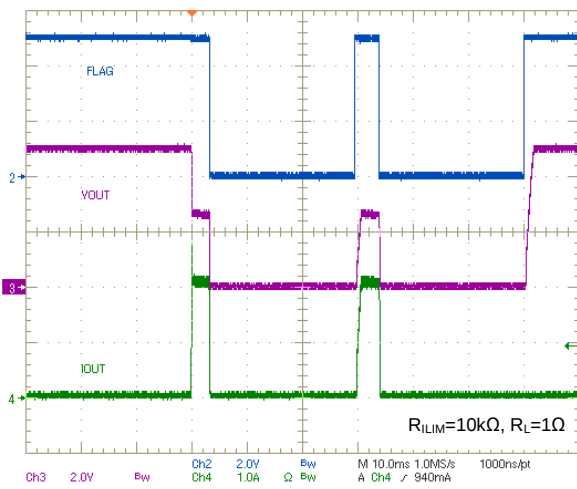
Over current protection: Auto-retry Mode
