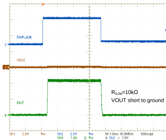
Enable with short circuit condition
