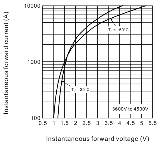
Fig.17 Forward voltage drop characteristics
