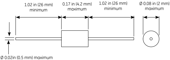
NTC Type TH dimensions
