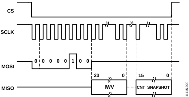
Figure 42. SPI Read Operation in Burst Mode
