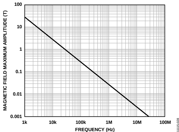
Figure 50. Maximum Allowable External Magnetic Field
