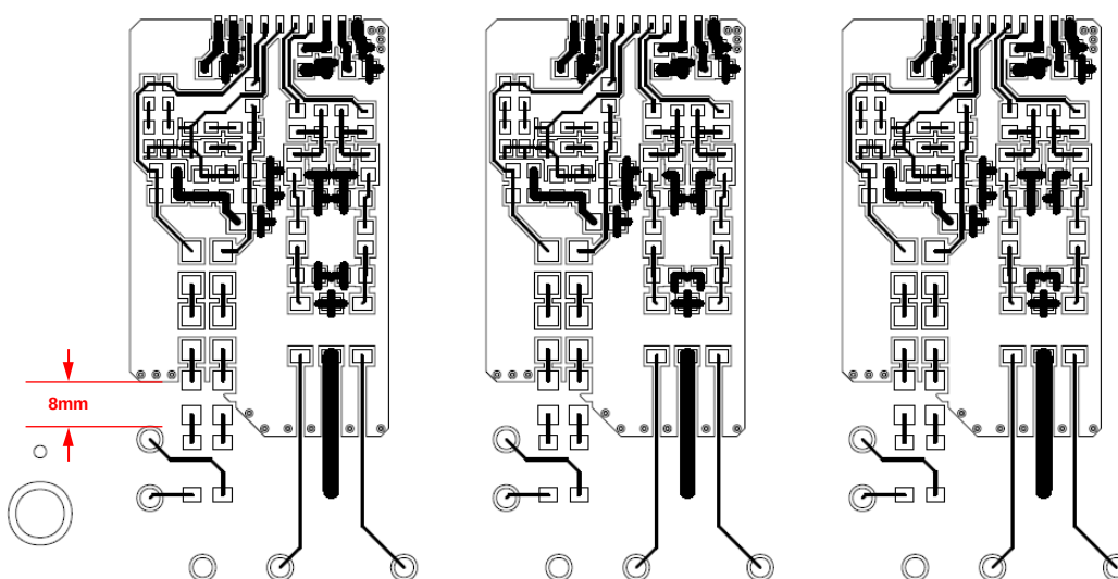
Figure 57. 4-Layer Circuit Board: Top Layer
