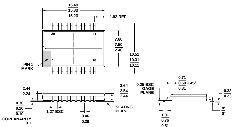
Figure 62. 20-Lead Standard Small Outline Package, with Increased Creepage [SOIC_IC] Wide Body (RI-20-1)
