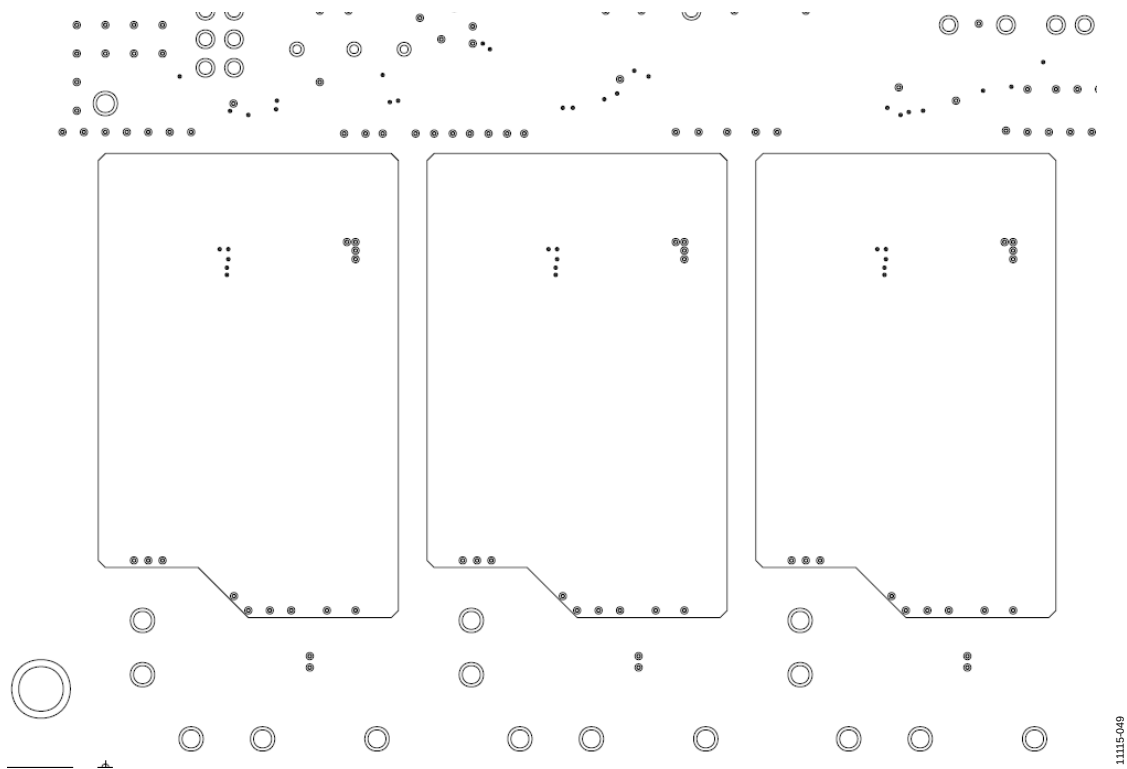
Figure 61. 4-Layer Circuit Board: Layer 3
