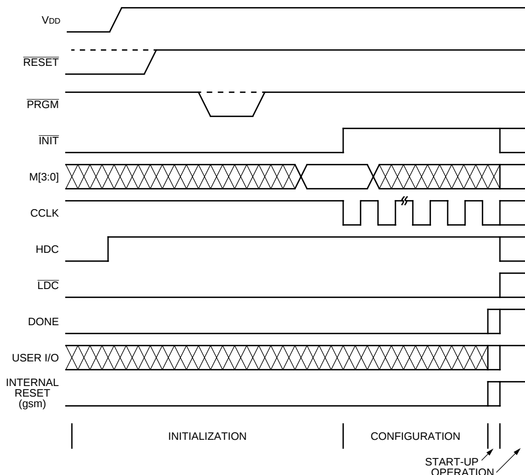
Figure 37. Initialization/Configuration/Start-Up Waveforms
