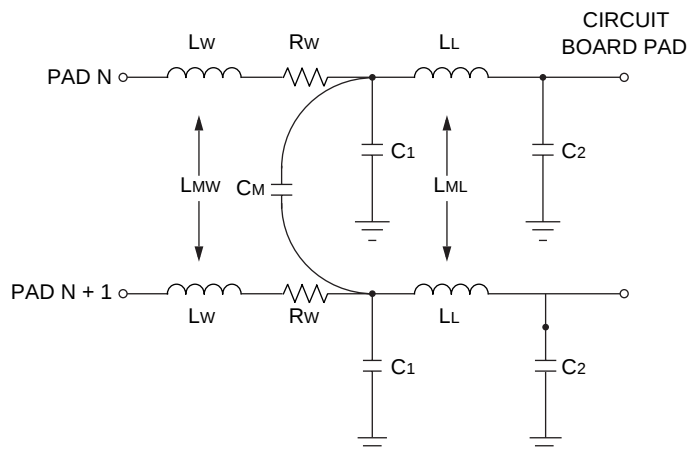
Figure 53. Package Parasitics
