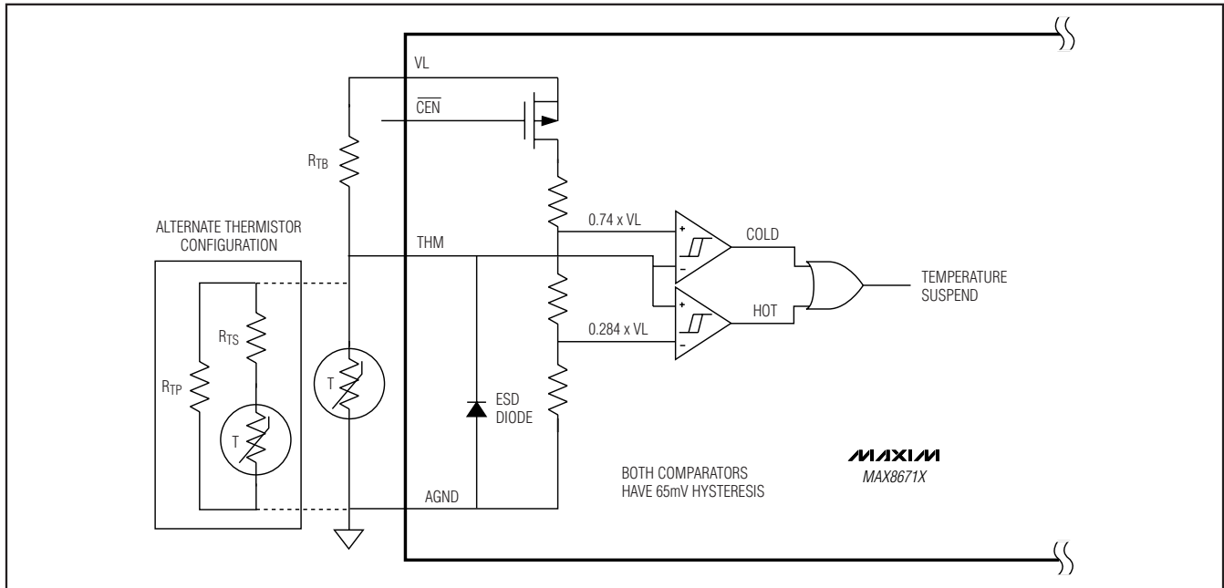
Figure 14. Thermistor Input
