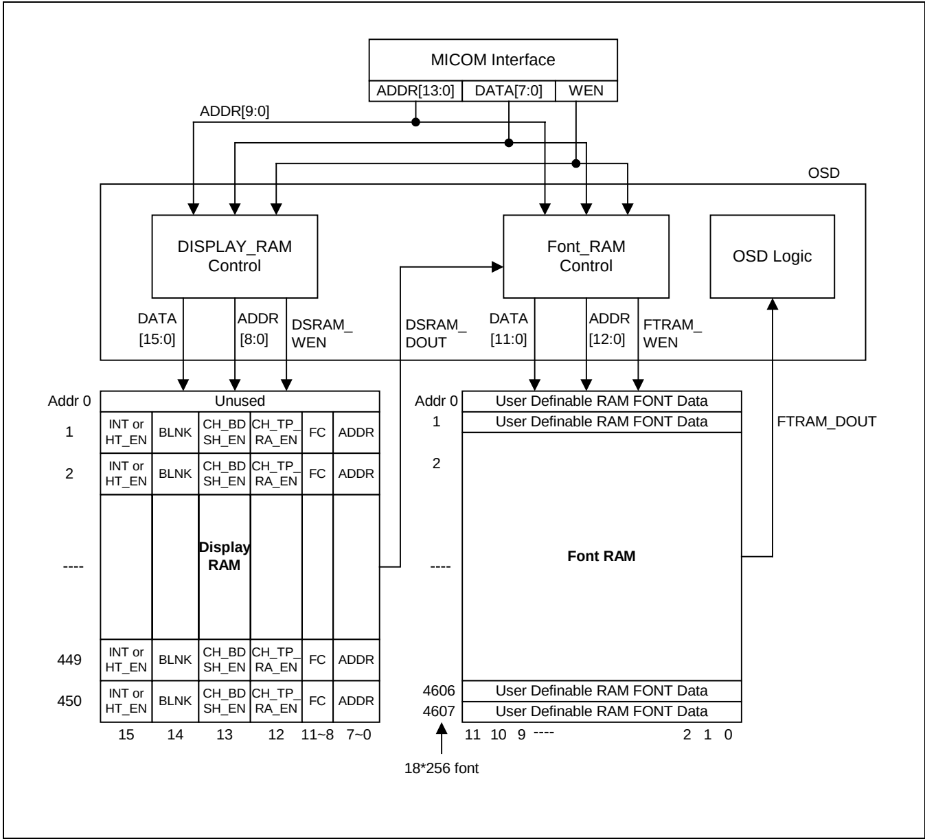
Figure 26. OSD RAM Structure
