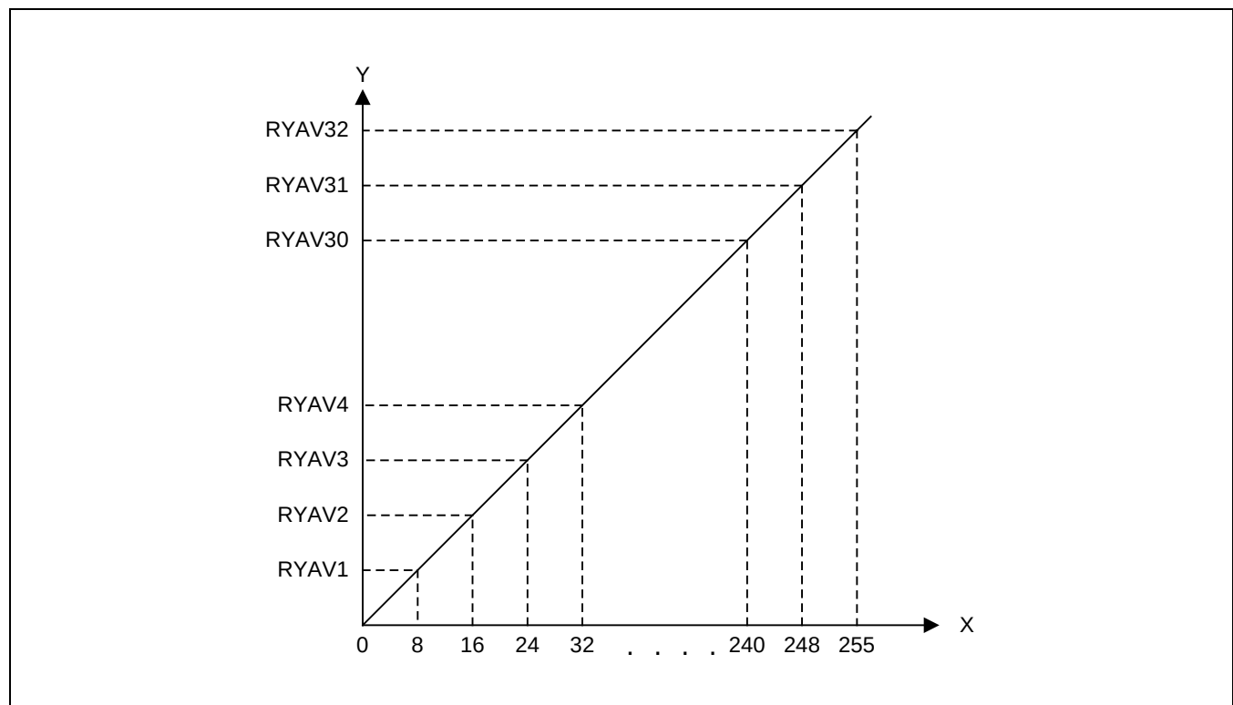
Figure 30. Gamma Graph
