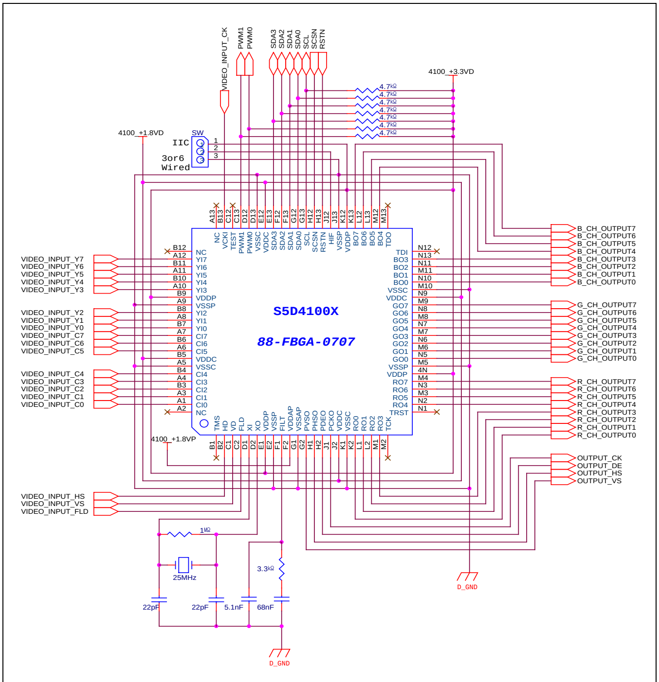
Figure 6. Solution Circuit for Application (FBGA)
