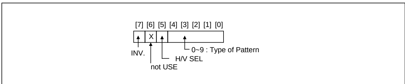
Figure 12. TP_SEL Register
