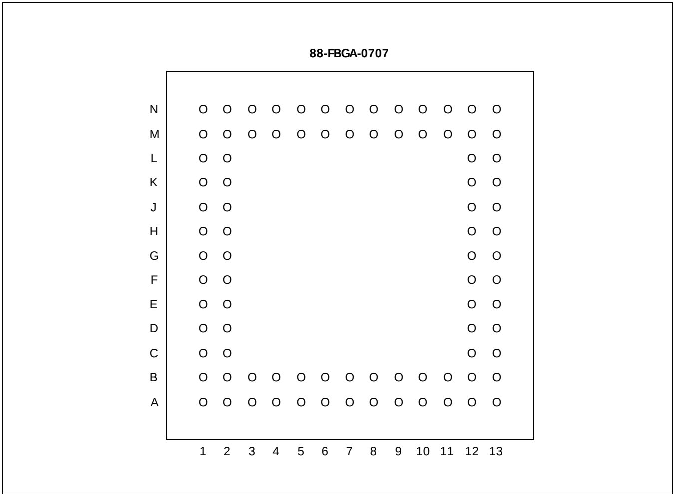
Figure 3. 88-FBGA-0707
