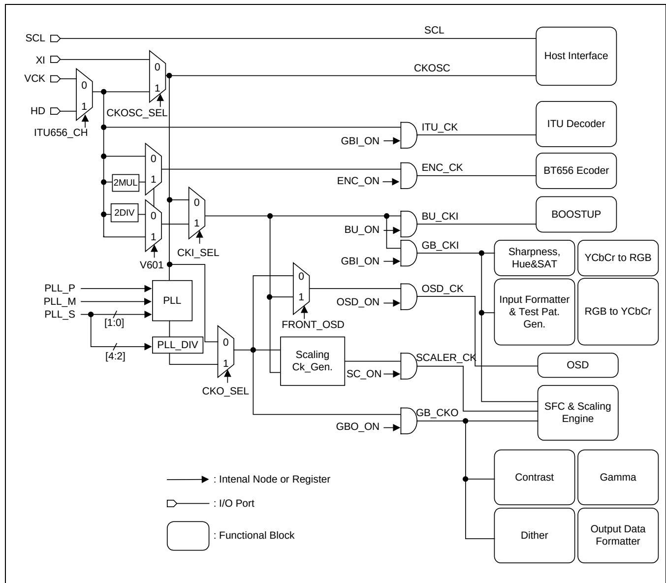
Figure 7. Clock Systems
