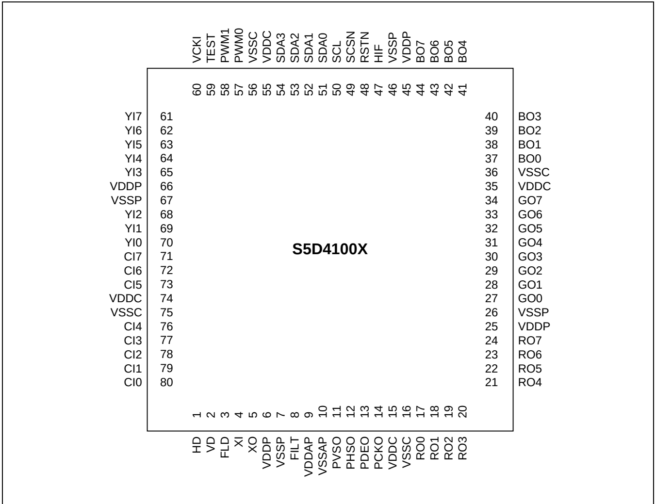
Figure 1. 80-TQFP-1212
