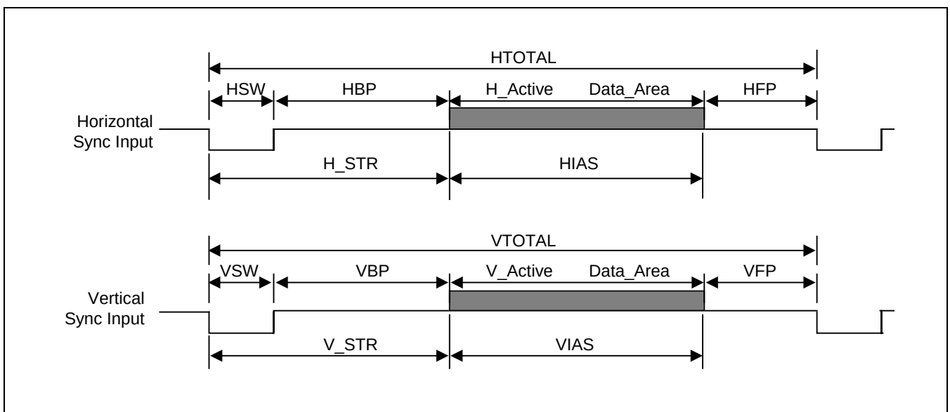
Figure 15. Input Timing
