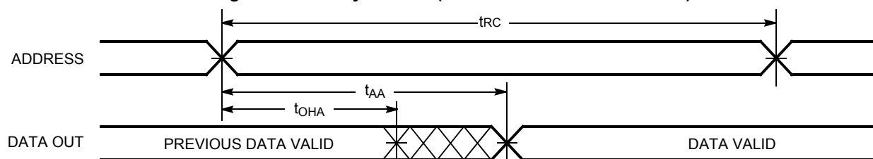
Figure 5. Read Cycle No. 2 ( \overline{\text{OE}} Controlled) [21, 22]
