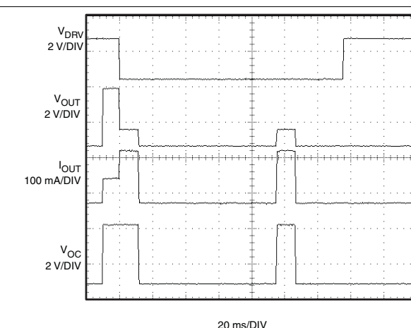
Figure 21. t_{RESTART} Response
