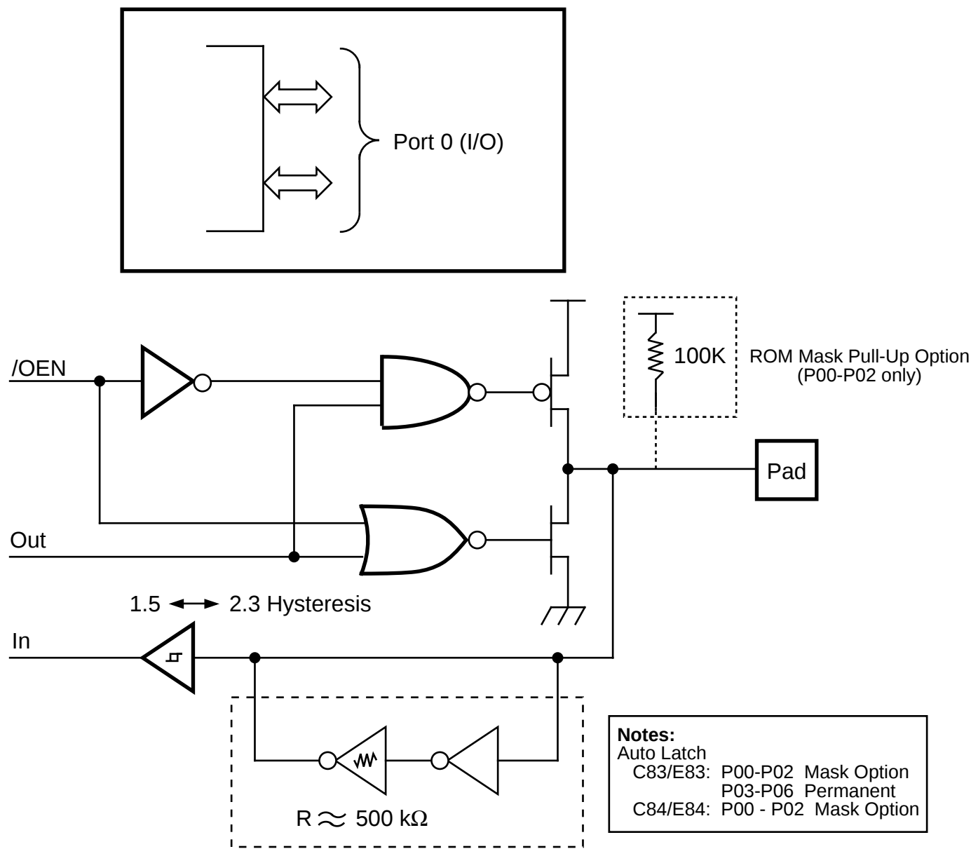
Figure 10. Port 0 Configuration
