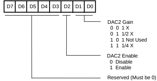
DACR2 Bank C, Register 5
