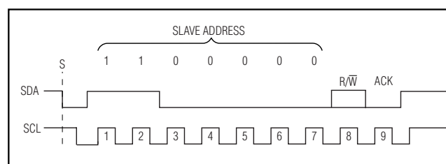
Figure 1. MAX2120 Slave Address Byte
