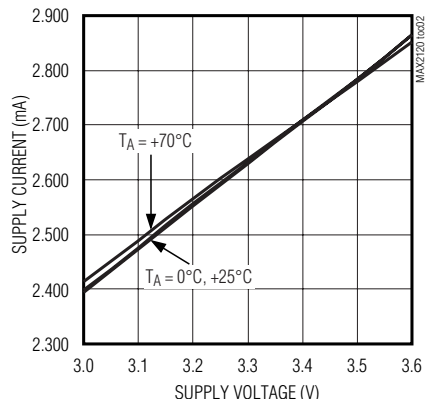
STANDBY MODE SUPPLY CURRENT vs. SUPPLY VOLTAGE
