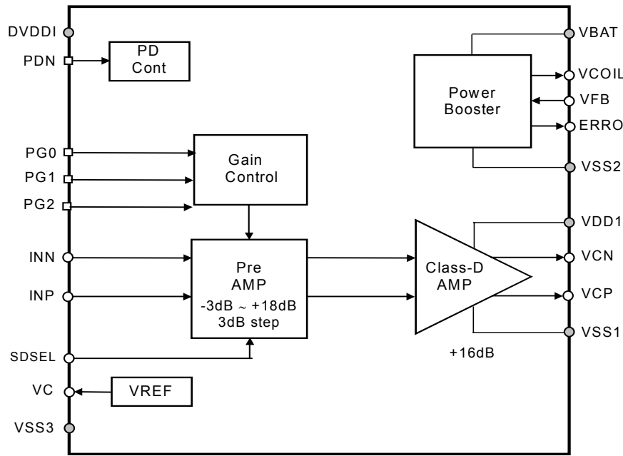
Figure. 1 Block Diagram
