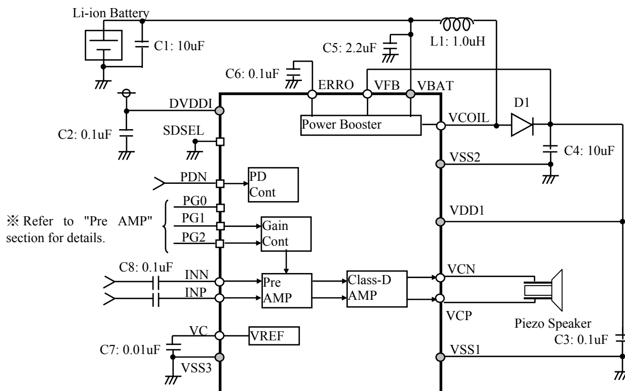
Figure. 17 External Components Examples : Differential Input with ac coupling capacitors at input
