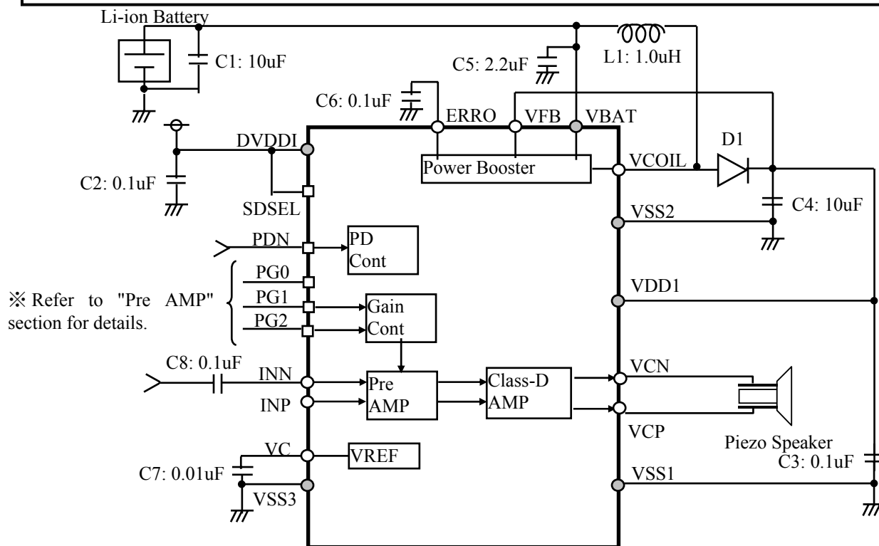
Figure. 16 External Components Examples : Single-ended Input
