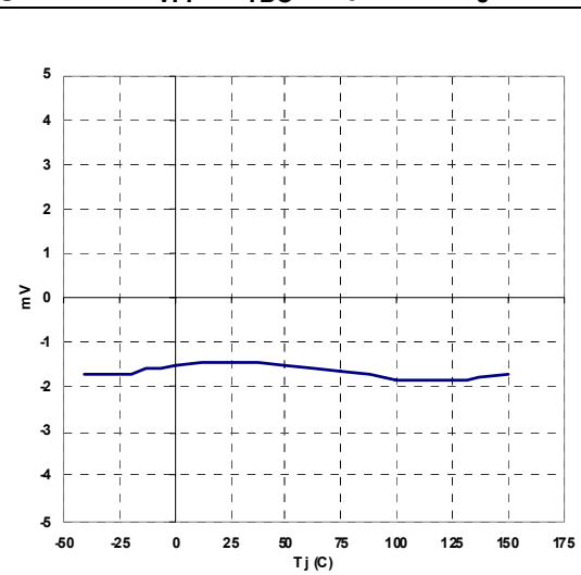
Figure 17. V_{VFF} - V_{TBO} dropout vs T_J
