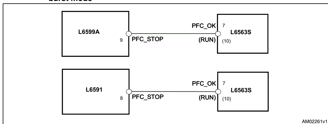
Figure 43. Interface circuits that let dc-dc converter's controller IC drive L6563S in burst mode
