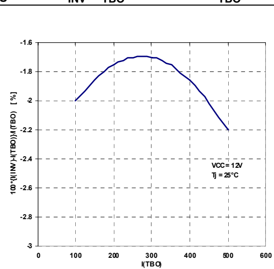
Figure 19. I_{INV} - I_{TBO} mismatch vs I_{TBO} current
