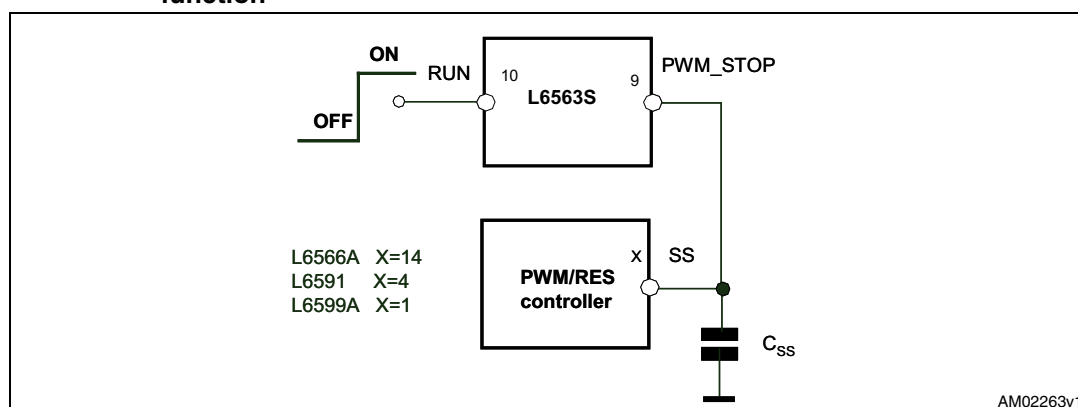
Figure 45. Interface circuits for power up sequencing when dc-dc has the SS function
