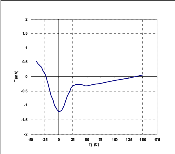
Figure 22. V MULTpk - V VFF dropout vs T J
