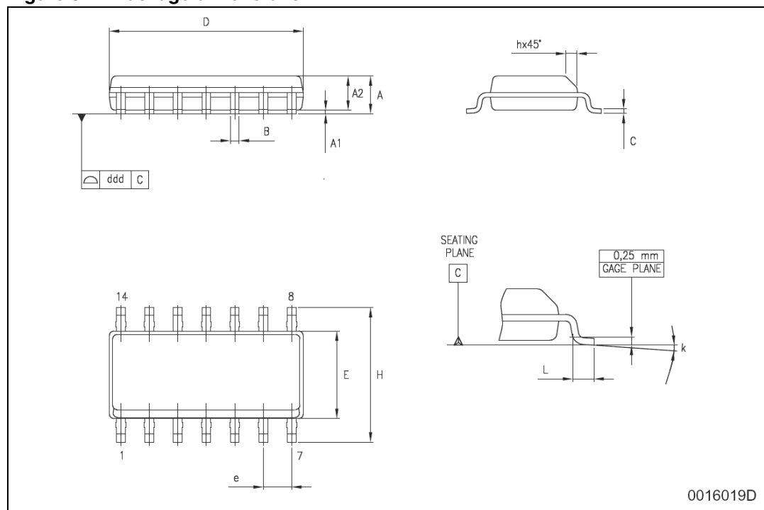
Figure 54. Package dimensions
