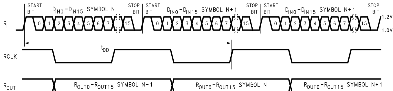
Figure 11. Deserializer Delay
