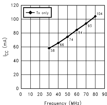
Figure 21. I_{\text{CC}} vs Freq (Tx only)
