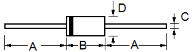
DO-201AE
