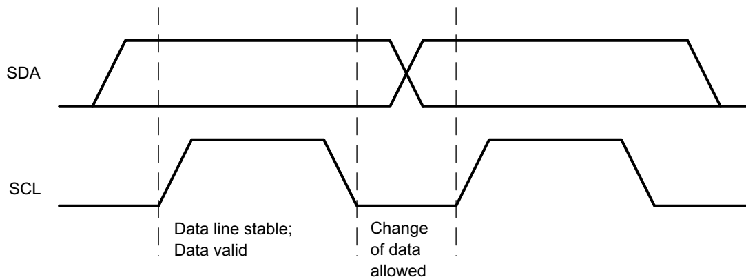
图 14. Bit Transfer on the I²C Bus
