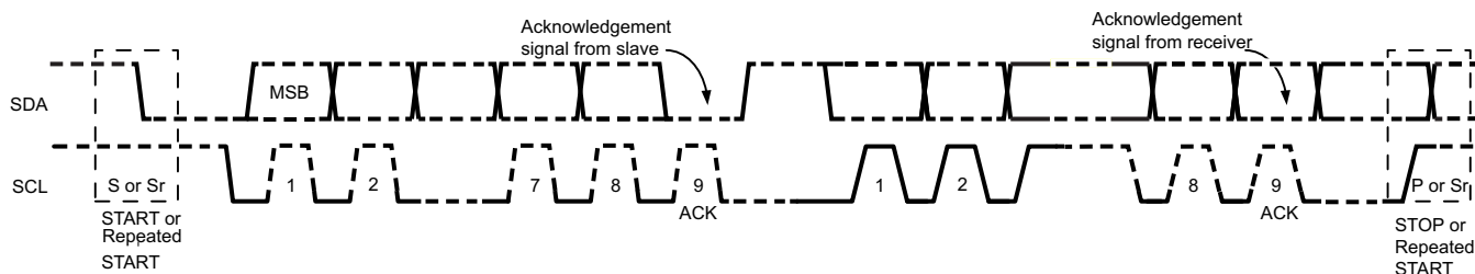
图 16. Data Transfer on the I²C Bus
