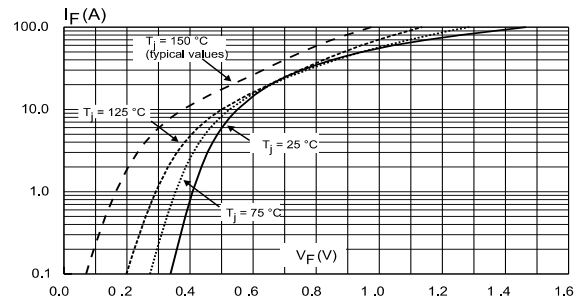
Figure 8: Forward voltage drop versus forward current (maximum values, per diode)
