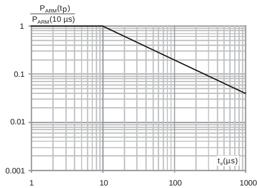
Figure 3: Normalized avalanche power deratings versus pulse duration ( T_j = 125\text{ °C} )
