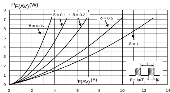
Figure 1: Average forward power dissipation versus average forward current (per diode)
