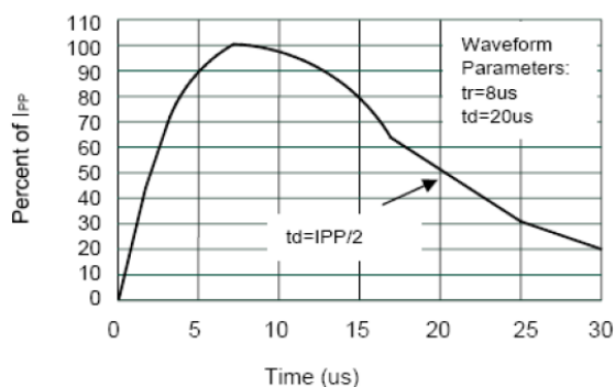
Pulse Waveform
