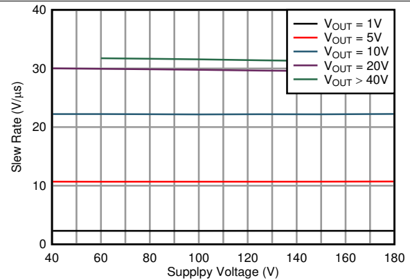
图 44. Slew Rate vs Supply Voltage (Inverting)
