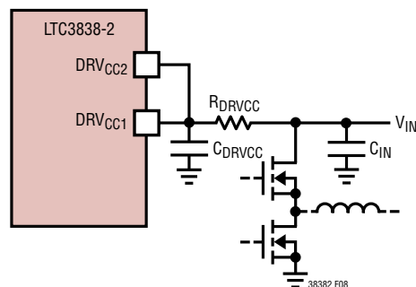
Figure 8. Setup for V_{IN} \leq 5.3\text{V}
