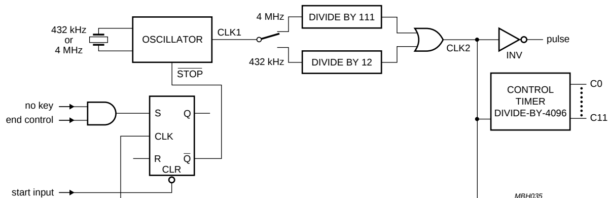
Fig.4 Timer schematic diagram.
