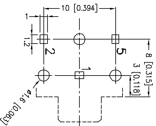
HOLE LAYOUT (TOP VIEW)
