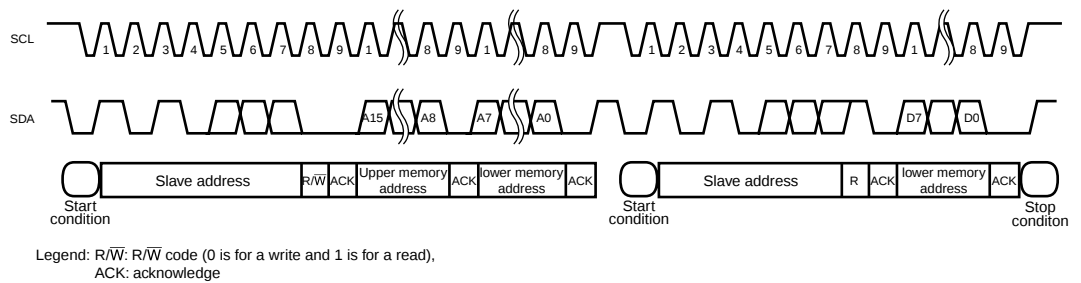
Figure 19.6 Random Address Read Operation
