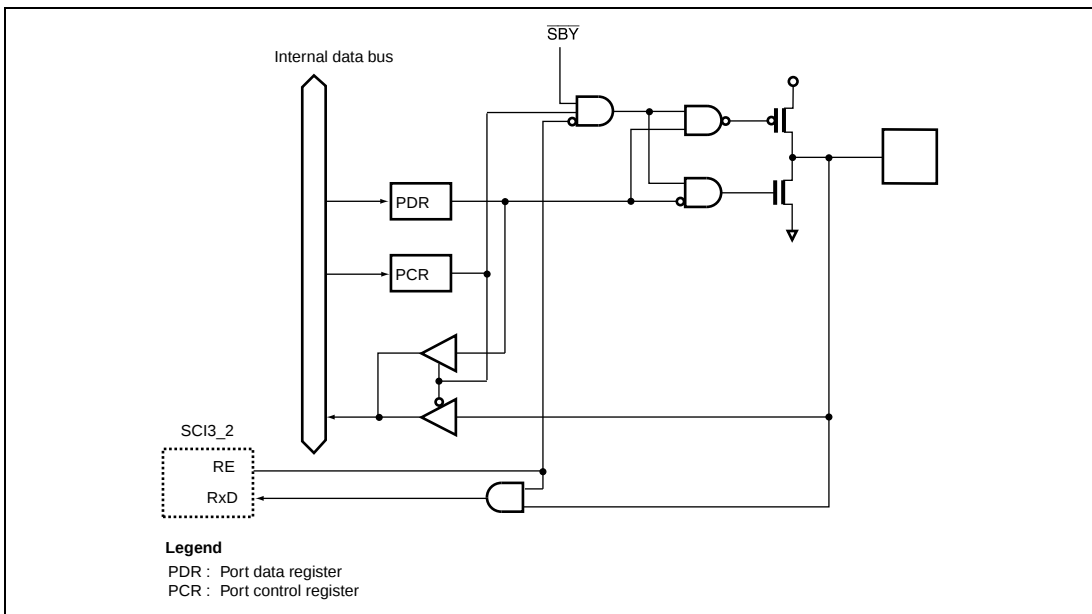
Figure B.19 Port 7 Block Diagram (P71)
