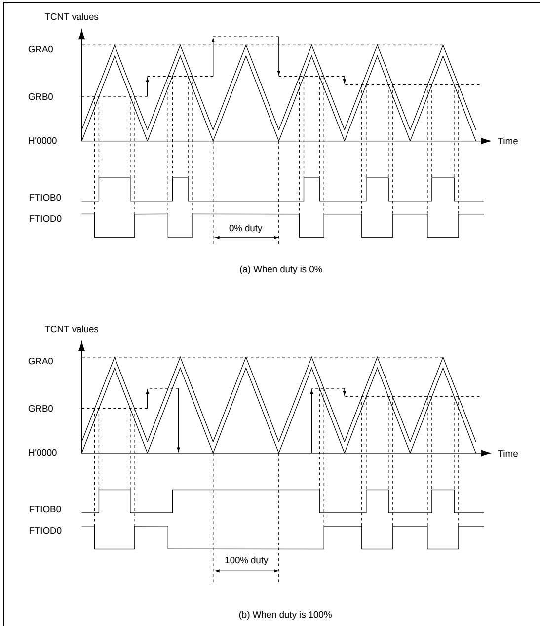
Figure 13.32 Example of Complementary PWM Mode Operation (2)
