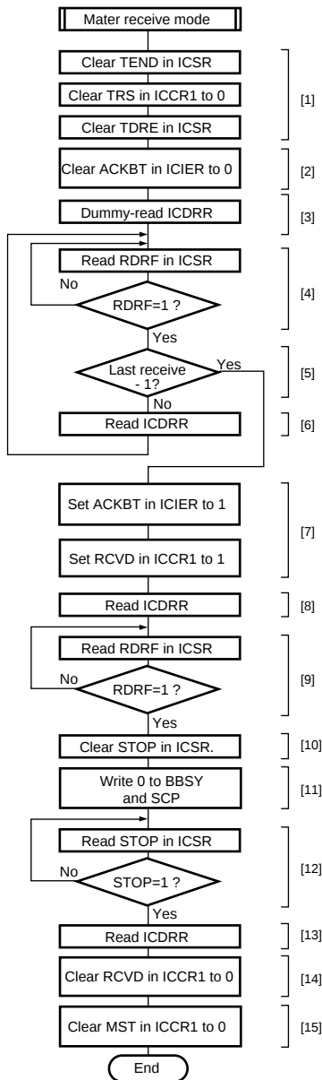
Figure 17.18 Sample Flowchart for Master Receive Mode
