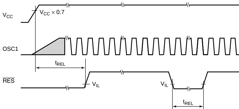
Figure 23.2 RES Low Width Timing
