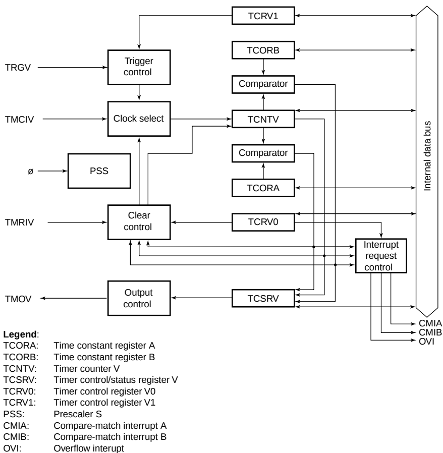
Figure 12.1 Block Diagram of Timer V
