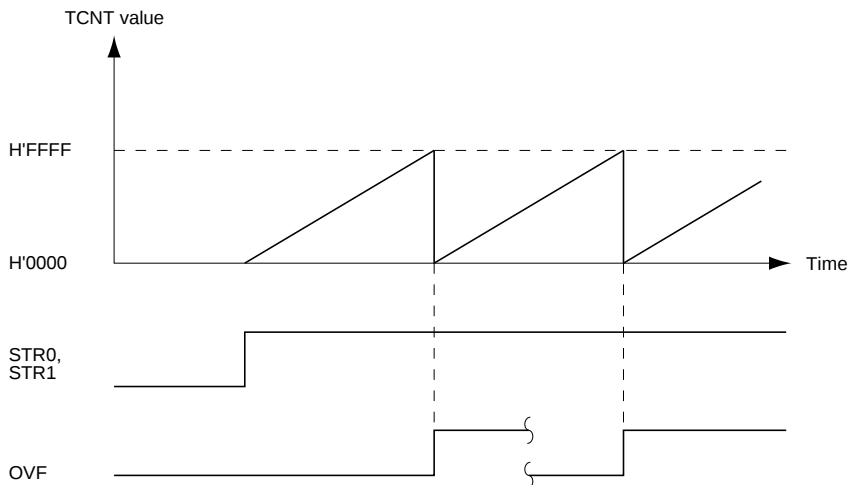
Figure 13.8 Free-Running Counter Operation
