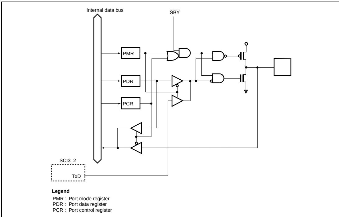
Figure B.18 Port 7 Block Diagram (P72)
