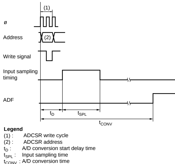
Figure 18.2 A/D Conversion Timing
