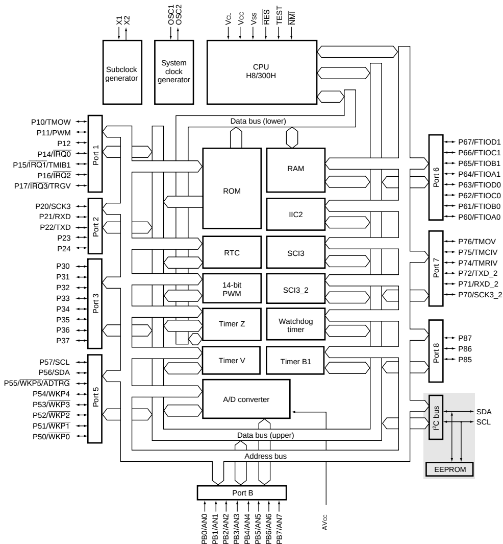
Figure 1.2 Internal Block Diagram of H8/3687N (EEPROM Laminated Version)
