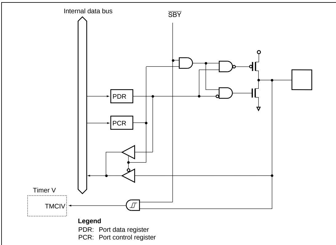
Figure B.16 Port 7 Block Diagram (P75)
