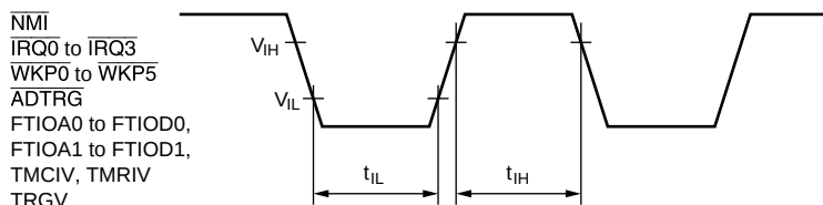
Figure 23.3 Input Timing
