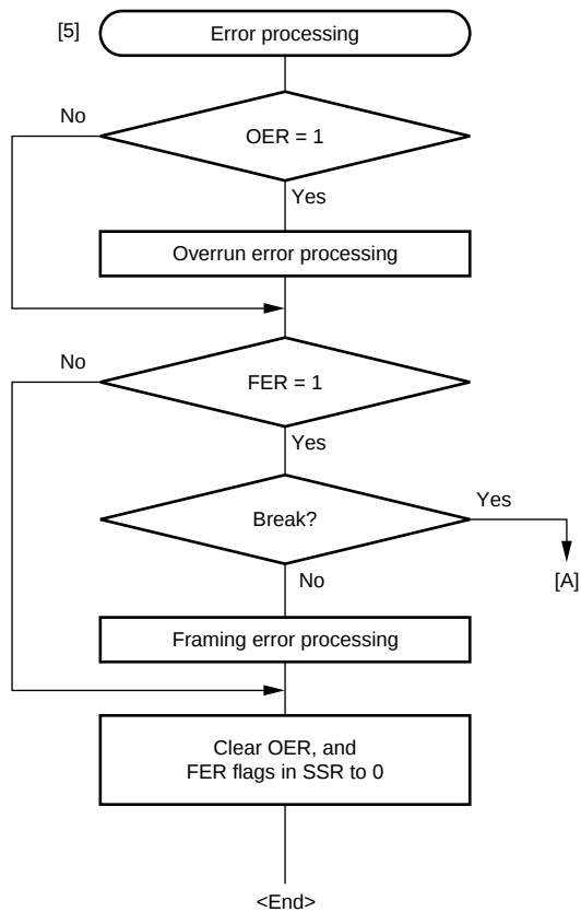
Figure 16.17 Sample Multiprocessor Serial Reception Flowchart (2)
