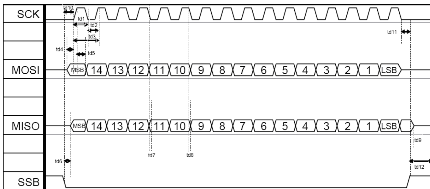
SPI Timing
