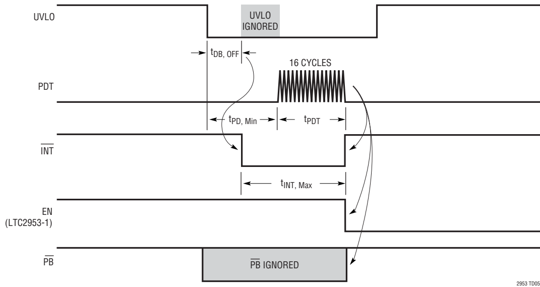
Figure 5. UVLO Power Down Timing: UVLO Low for t > (t_{PD, Min} + t_{PD, Max})
