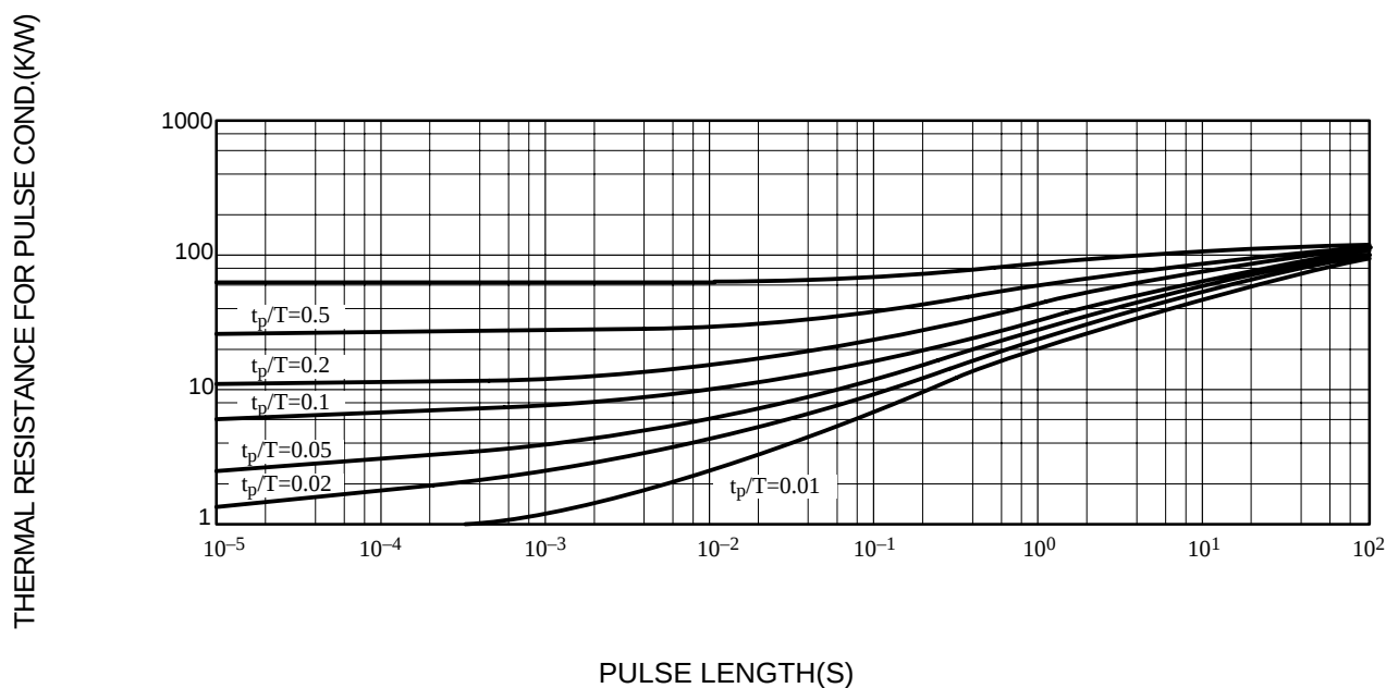
FIG.3 – THERMAL RESPONSE
