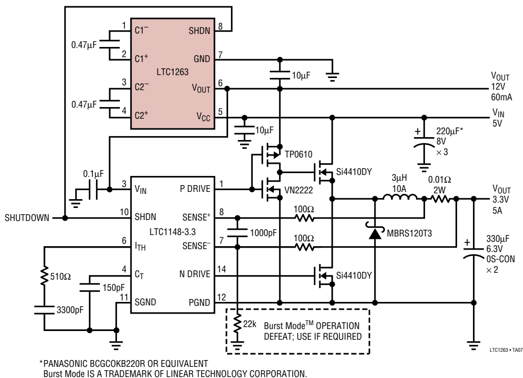
5V to 3.3V/5A Converter with 12V/60mA Auxiliary Output
