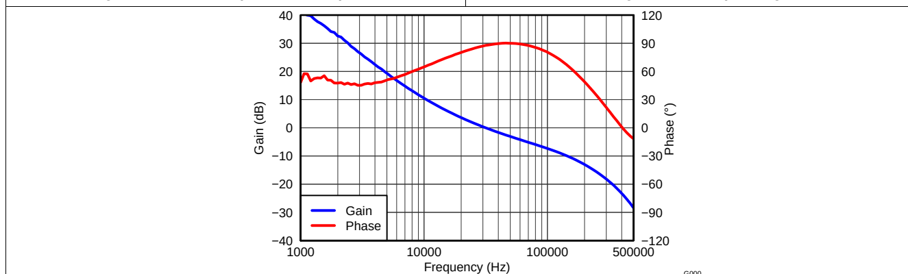
Figure 5. V_{OUT} = 1.8 V, I_{OUT} = 2 A, C_{OUT1} = 47 \mu F ceramic, C_{OUT2} = 100 \mu F POSCAP, f_{SW} = 1 MHz
