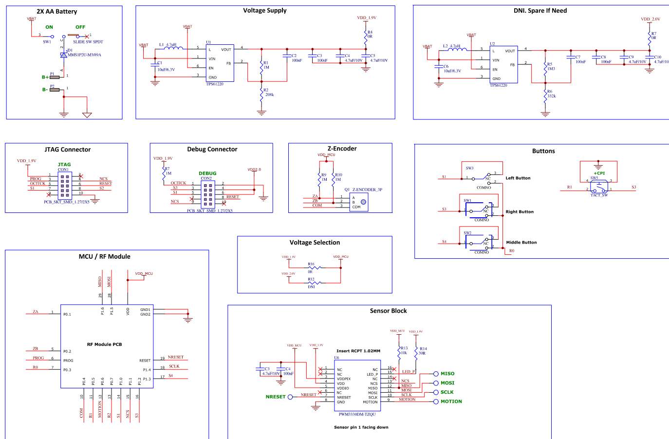
Figure 5. Schematic diagram for interface between PMW3330DM-TZQU and microcontroller in a wireless solution
