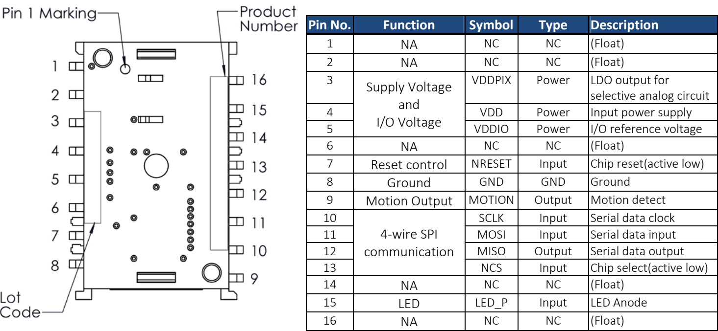
Figure 1. Device output pins
