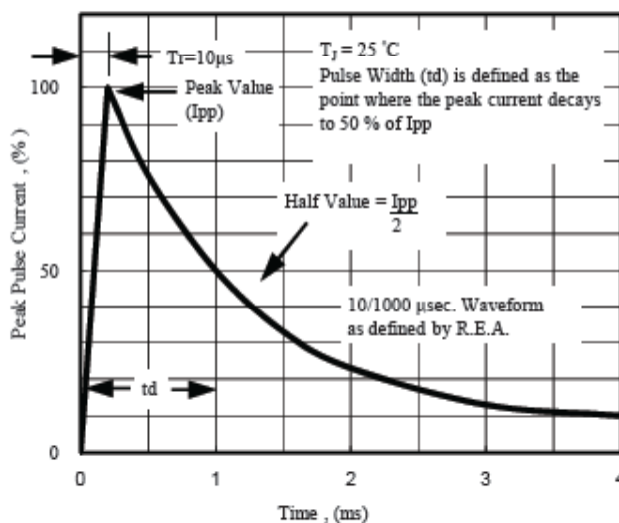
Fig. 5 - Pulse Waveform
