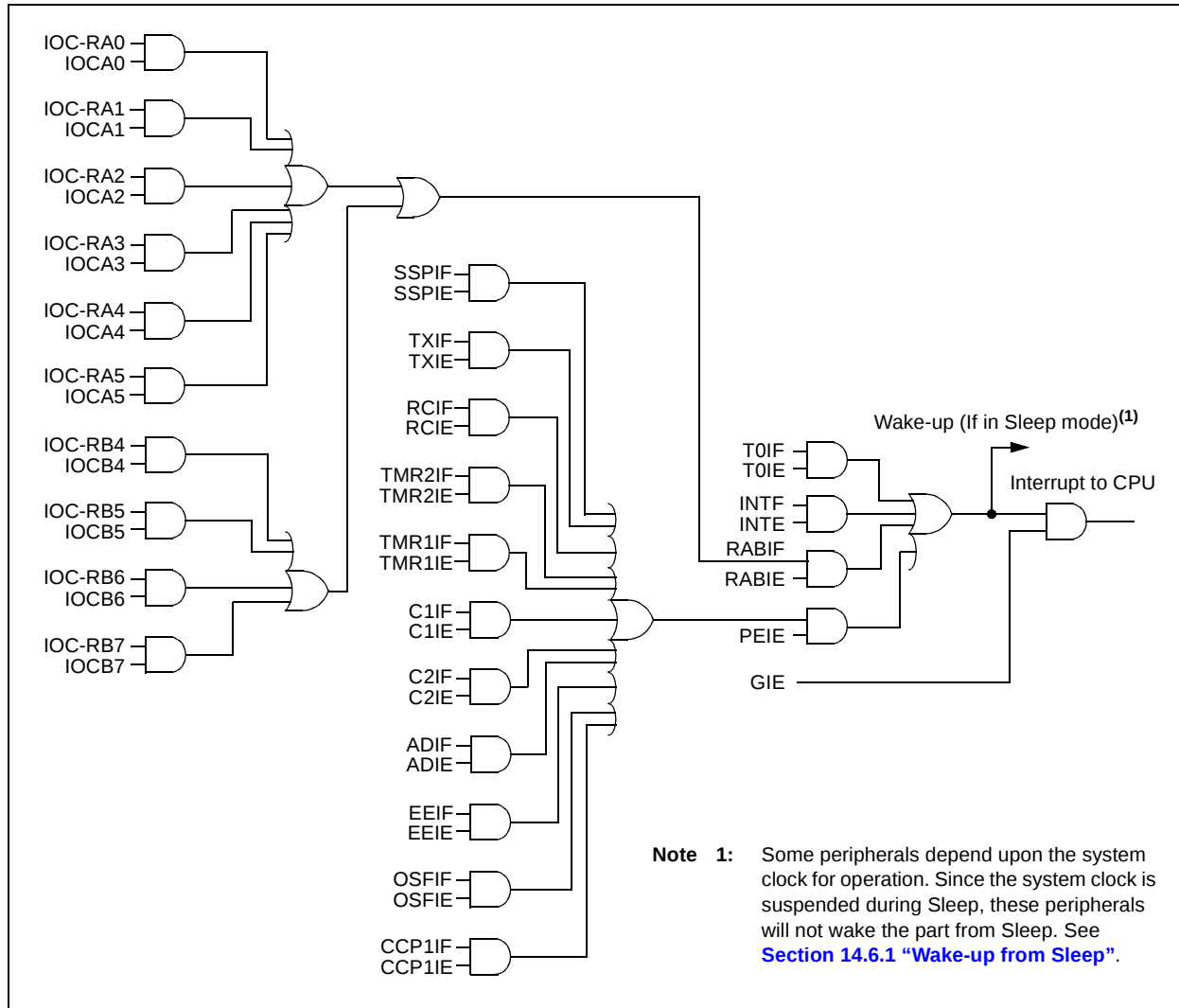
FIGURE 14-7: INTERRUPT LOGIC
