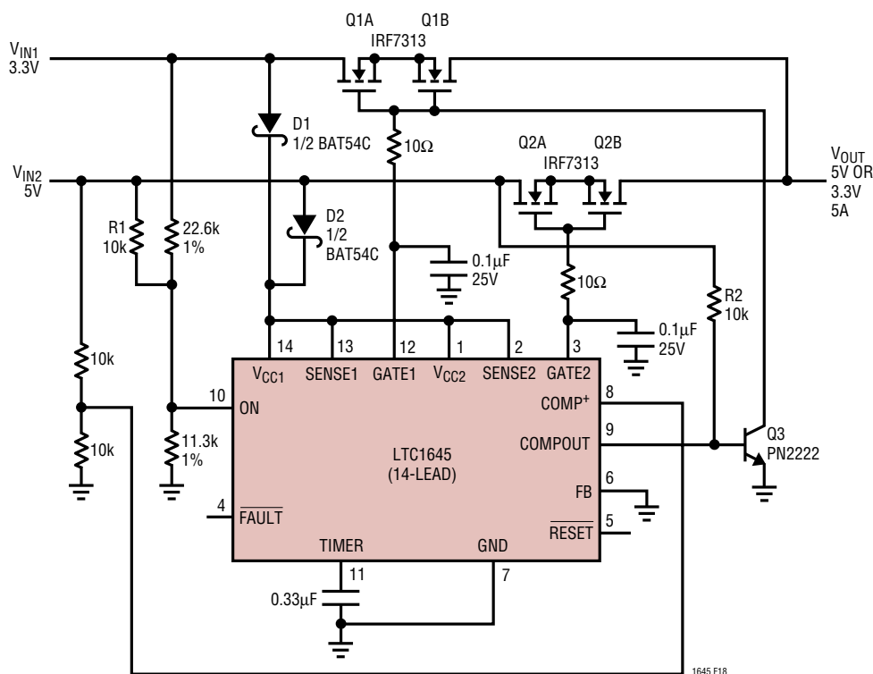
Figure 18. Power Supply Multiplexer
